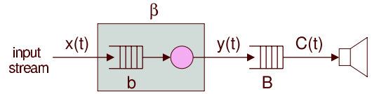
Fig. 1. A node with a processing element and an internal buffer of size b , processing an input stream and feeding the processed stream into a playout buffer of size B .
