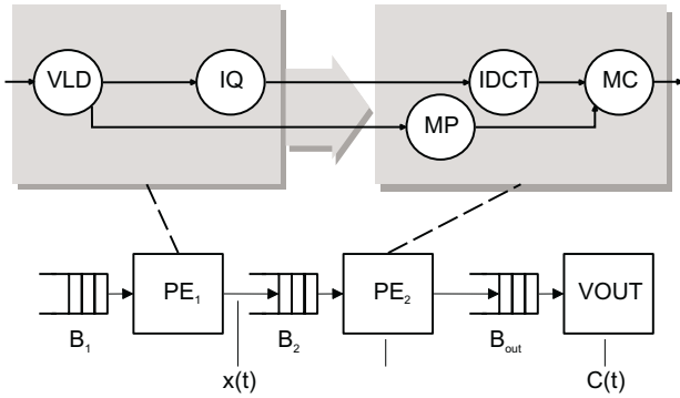
Fig. 2. Mapping the MPEG-2 decoder application onto a multiprocessor SoC.
