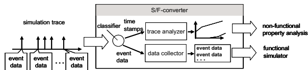
Figure 5. Interface between formal analysis method and simulator: the S/F-converter.
